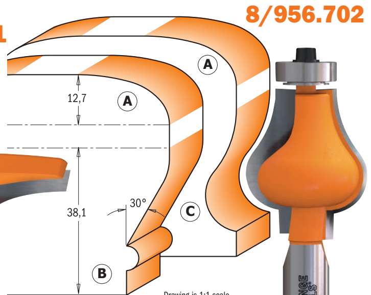
Drawing is 1:1 scale
