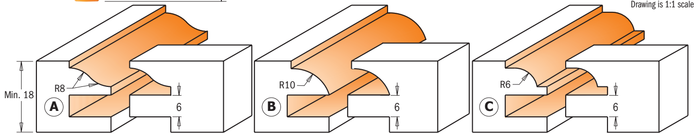
Drawing is 1:1 scale
