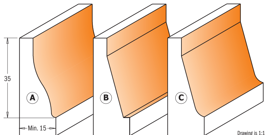
Drawing is 1:1 scale
